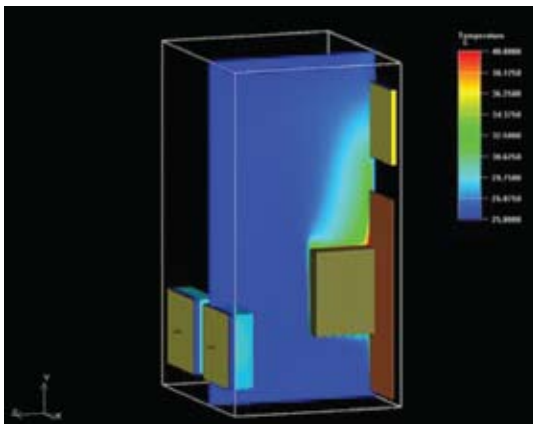
Temperature Distribution, parallel fans.
