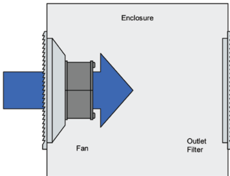
Impeded airflow. Air displacement with outlet filter including standard filter mat.
