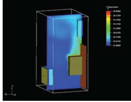
Temperature Distribution, fans in series.
