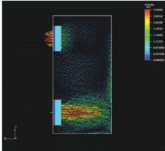
Screen shot of a CFD calculation.
