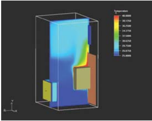
Temperature Distribution, single fan.
