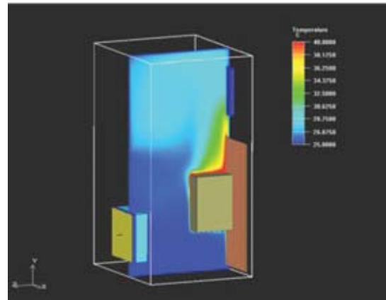
Temperature Distribution, single fan.
