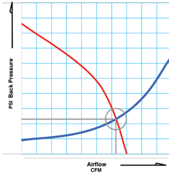
Fan curve with impedance.
